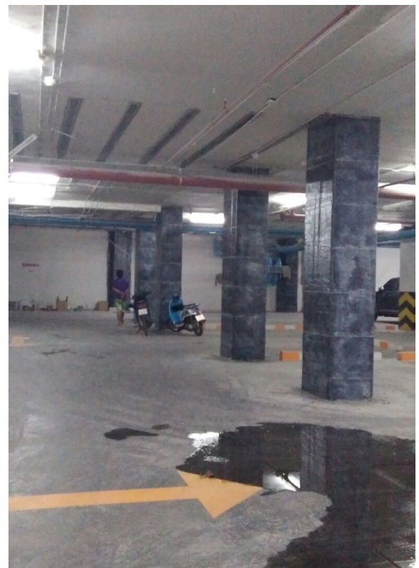
Build Wrap Pro 300, apply on Column
