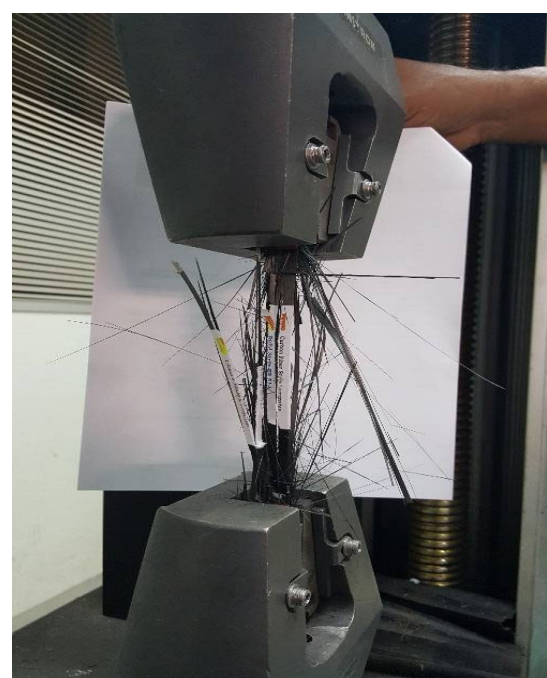
Testing Equipment, Method of Tester Installed, Once Tested the CFRP Cured Laminates Breaking
