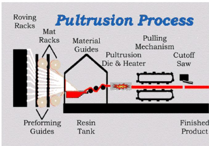
Solid Rod Bar Pultrusion Process
